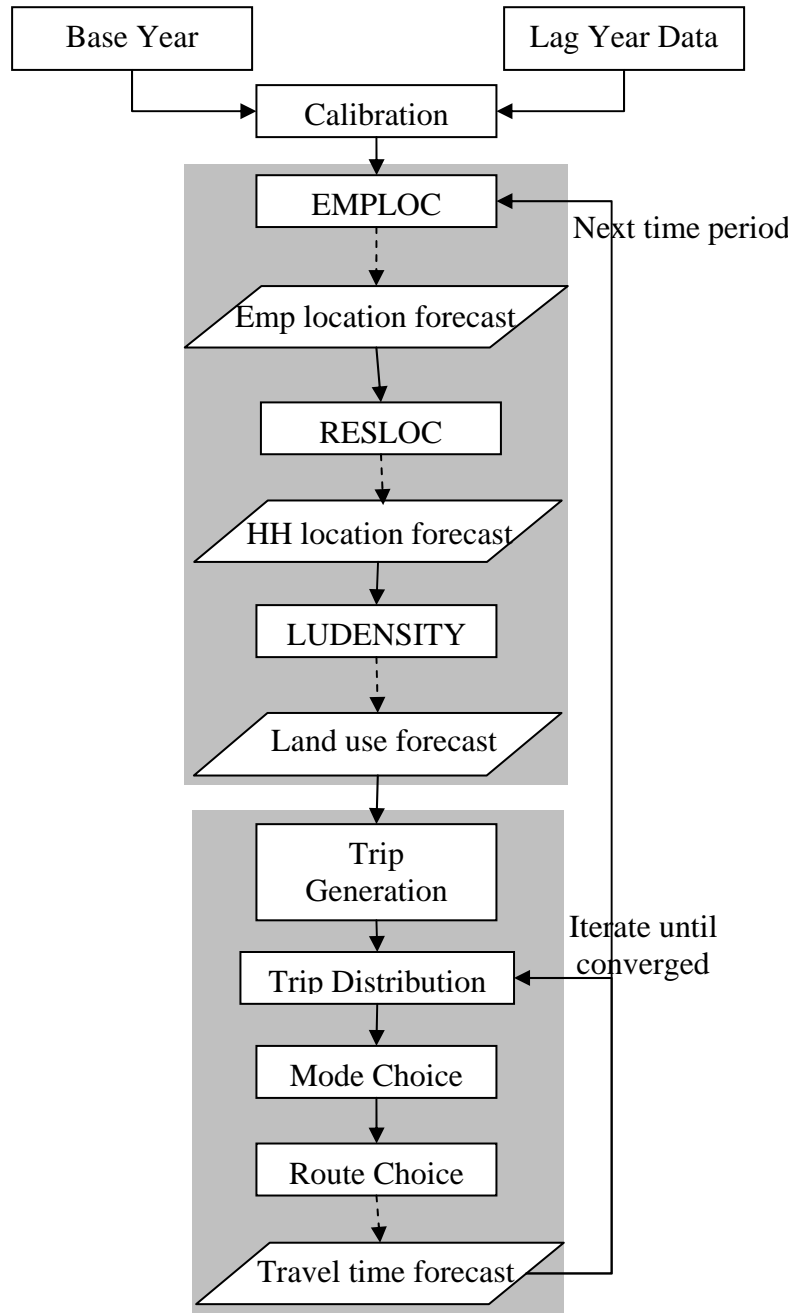
FIGURE 1 Diagram of ITGLUM
